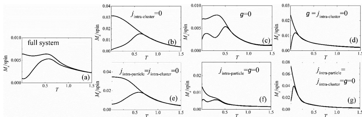
Fig. 5 Monte Carlo simulation results for the ZFC/FC magnetisation curves as a function of temperature for the albumin coated system 14 (a) and for the cases where we switch off: only the exchange intra-cluster interactions among all the nanoparticles in a cluster ( j_{\text{intra-cluster}} = 0 ) (b), only the dipolar inter-particle interactions among all the nanoparticles ( g = 0 ) (c), the dipolar and intra-cluster interactions ( g = j_{\text{intra-cluster}} = 0 ) (d), and switching off all the exchange interactions ( j_{\text{intra-particle}} = j_{\text{intra-cluster}} = 0 ) (e) or both the intra-particle and the dipolar interactions ( j_{\text{intra-particle}} = g = 0 ) (f) and all the inter-particle, intra-cluster and intra-particle interactions ( j_{\text{intra-particle}} = j_{\text{intra-cluster}} = g = 0 ) (g).
